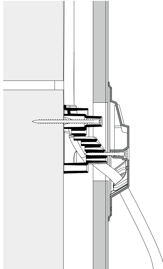
Larger Plasterboard Void Offsets >17mm
