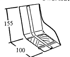
GW298RH
