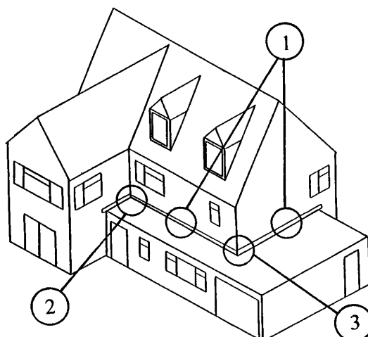
G953 DIAMOND WEEP OR G950 WEEP VENT
