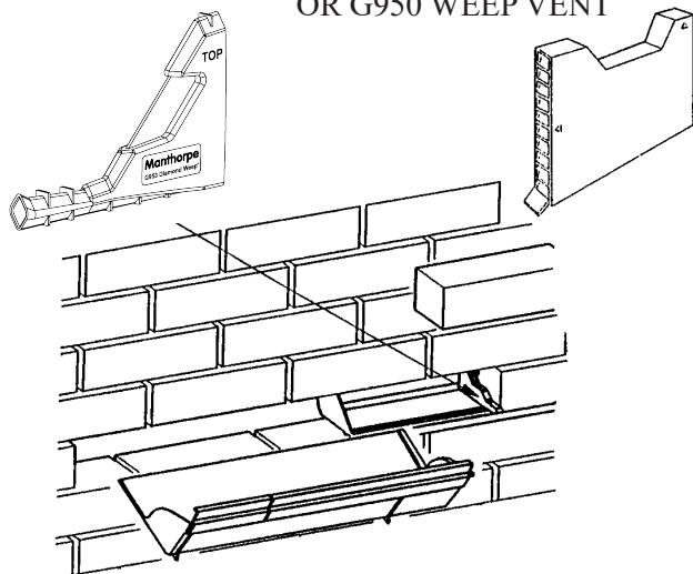
G951 DIAMOND WEEP OR G950 WEEP VENT
