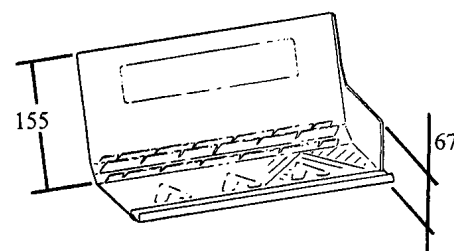
GW292 LH INTERMEDIATE TRAY
