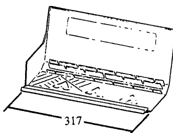
GW291 RH INTERMEDIATE TRAY
